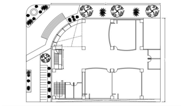
Planos PB
